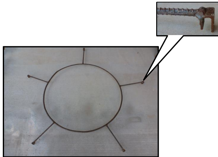
Figure 1. Rebar Jig
